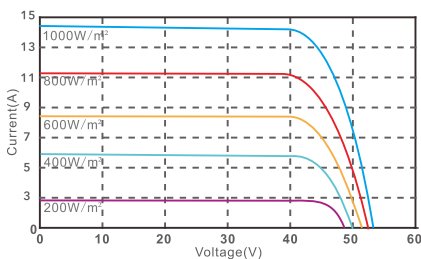
I-V characteristics at different irradiances (reference to 615 W)
