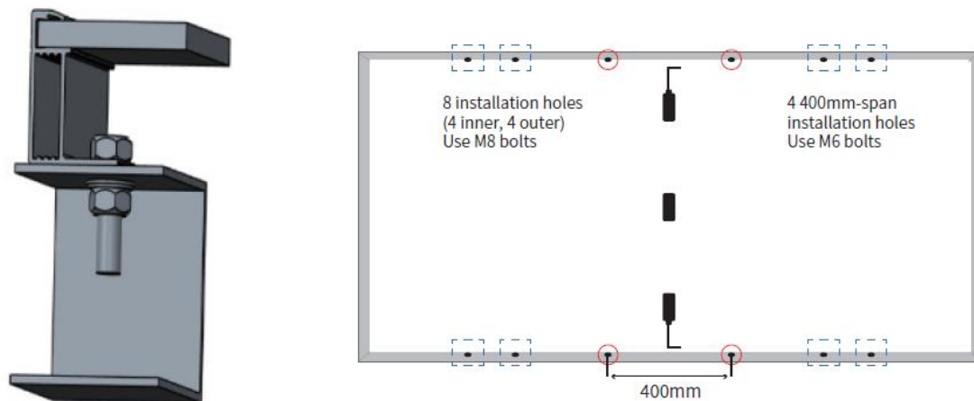
Figure 1 Schematic diagram1 of monofacial module with bolt Installation
