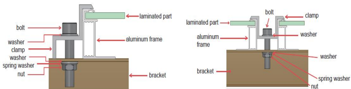
Figure 3 Clamp Installation of Monofacial Module
