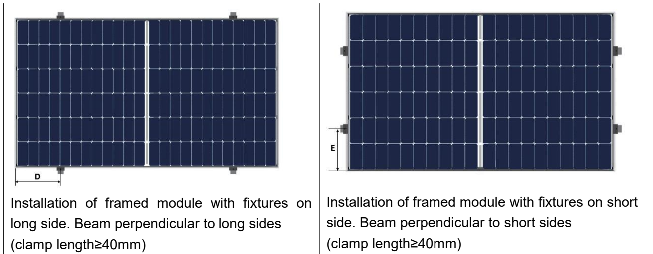
Figure 4 Monofacial Module Installation Annex
