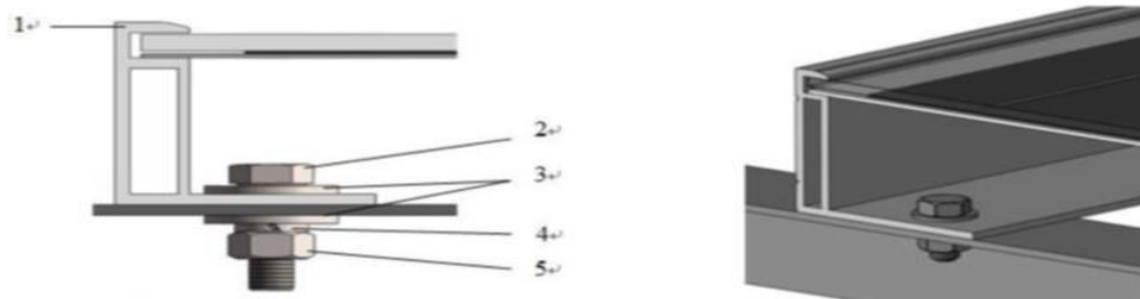
Figure 1 Schematic diagram1 of monofacial module with bolt Installation
